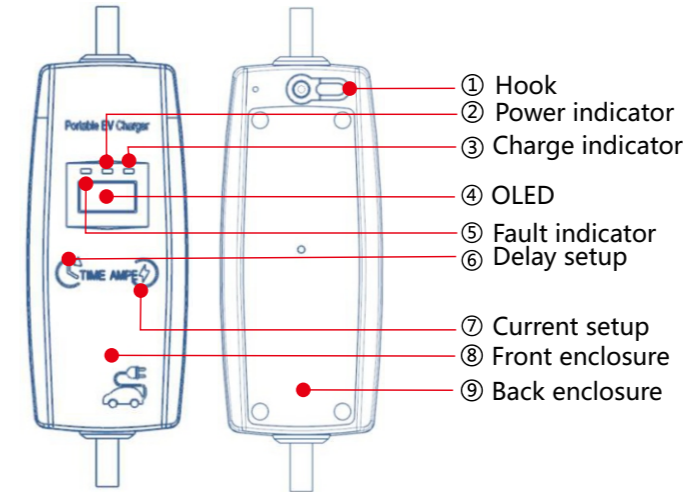
Figure 2 Front and Back of IC-CPD
